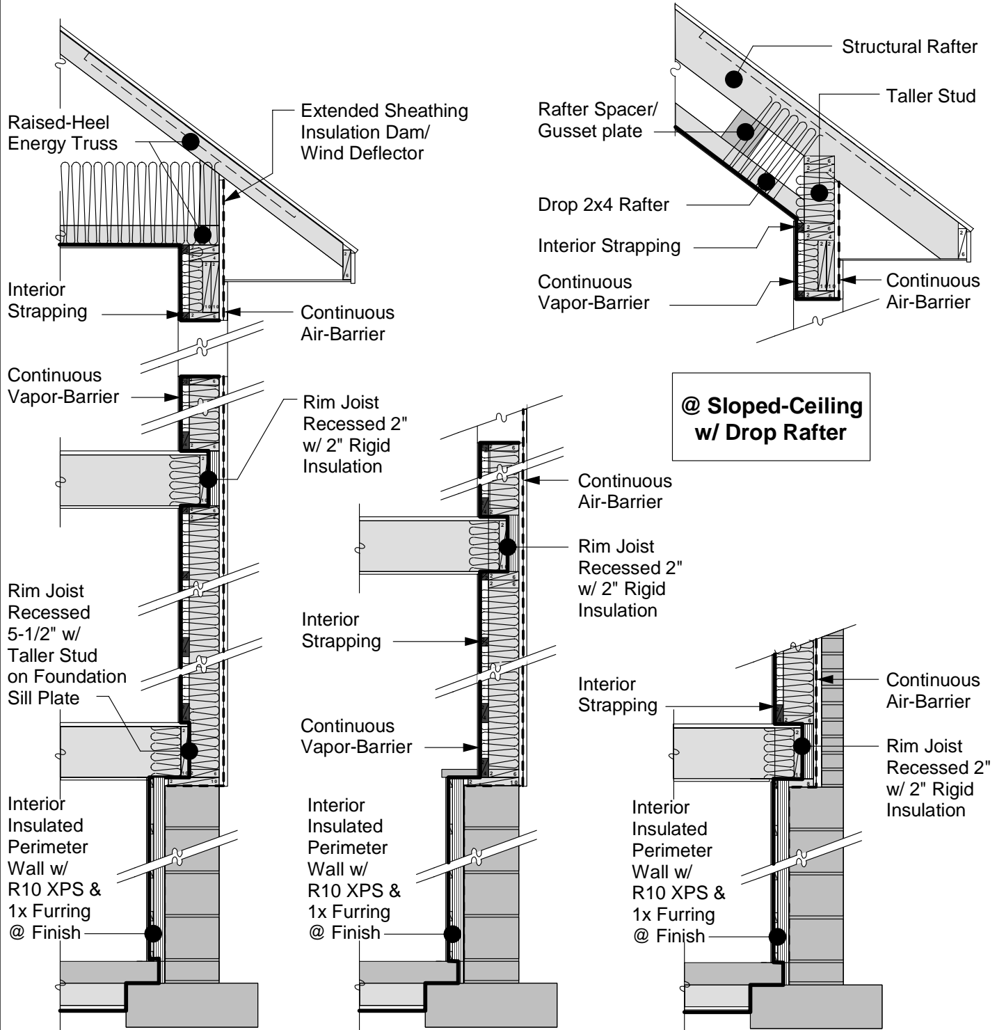
@ Strapped-Wall w/ Full-Height Foundation & Upper Floor Level
